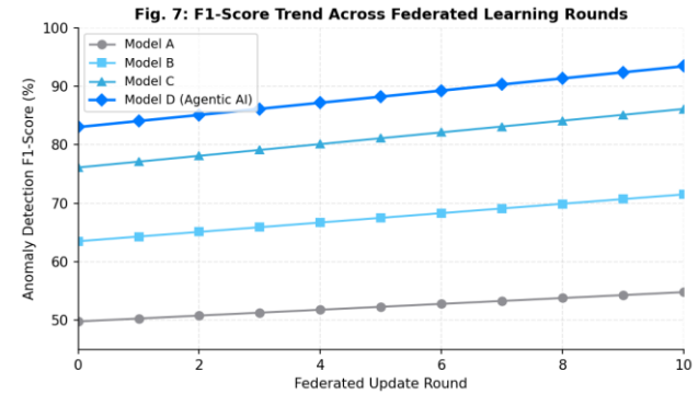
Fig. 7: F1-Score Trend Across Federated Learning Rounds
