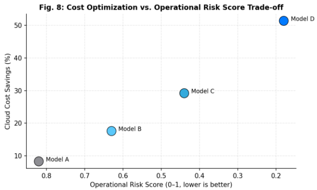
Fig. 8: Cost Optimization vs. Operational Risk Score Trade-off
