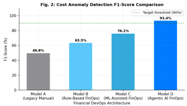
Fig. 2: Cost Anomaly Detection F1-Score Comparison
