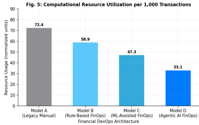
Fig. 5: Computational Resource Utilization per 1,000 Financial Transactions (normalized units)
