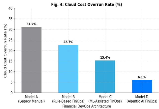
Fig. 4: Cloud Cost Overrun Rate (%)
